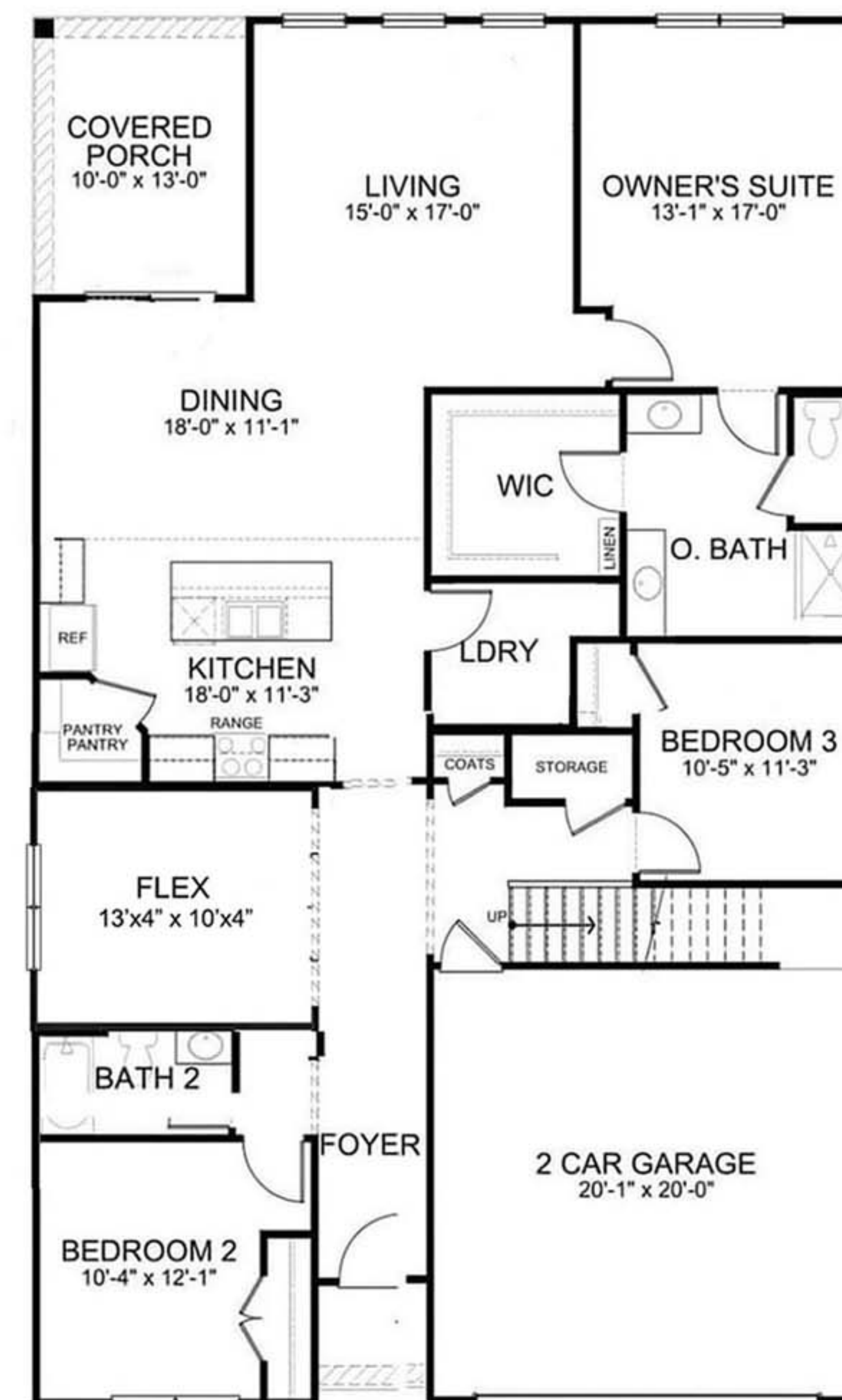
FIRST FLOOR
