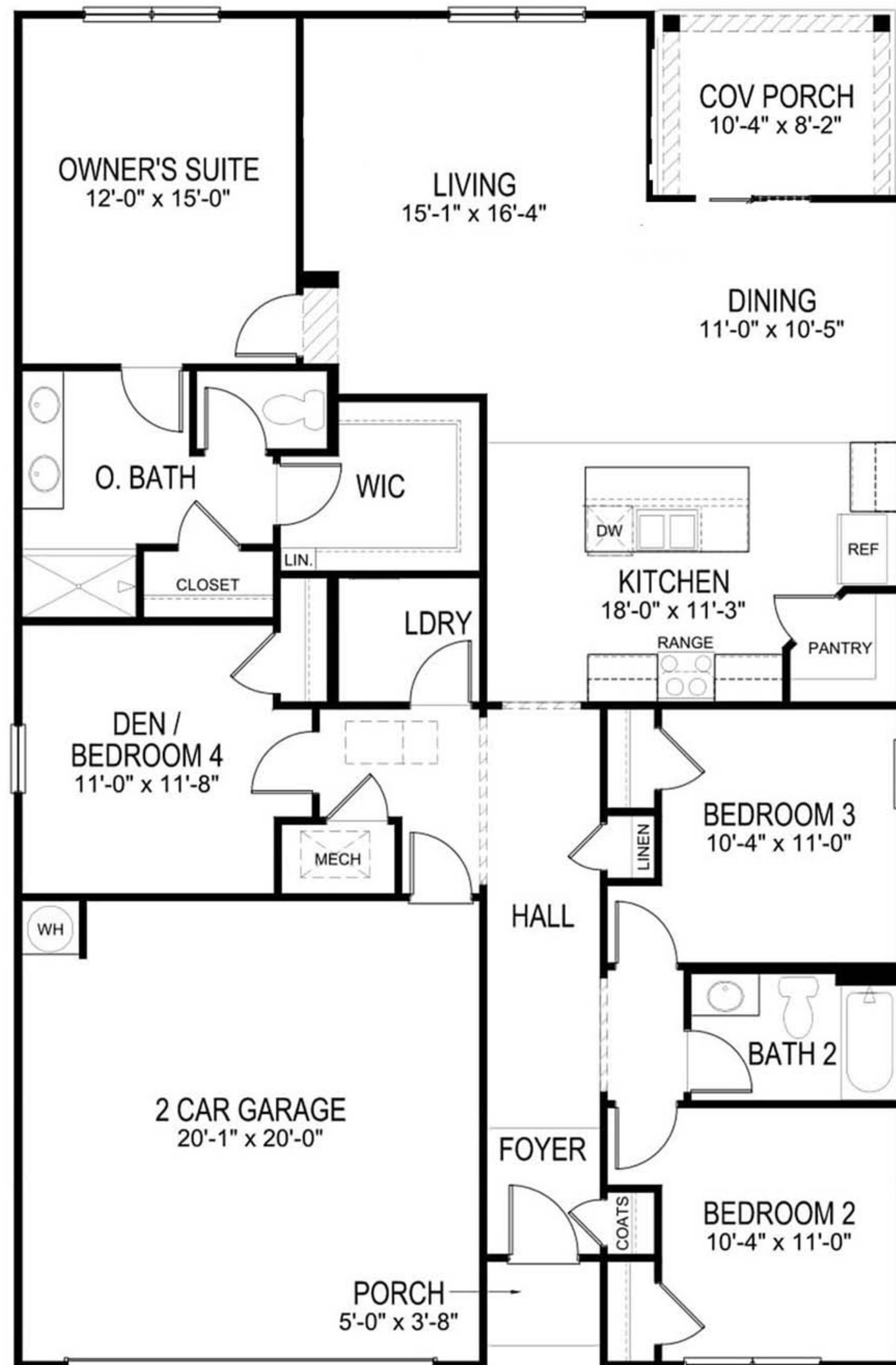
FIRST FLOOR
