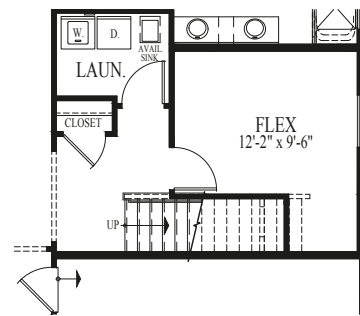
Main Level with Available Upper Level
