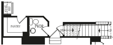
Main Level with Available Basement
