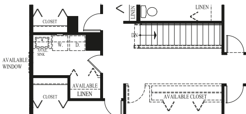
Upper Level with Available Basement
